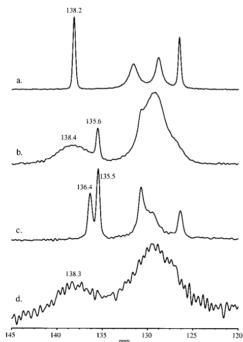
Figure 14. Phenyl region of the ^{13}\text{C} CP/MAS NMR spectra acquired with TOSS of: (a) neatame monohydrate; (b) neatame anhydrate (monohydrate was placed under reduced pressure ( \sim 100 Torr) at 60^\circ\text{C} for approximately 12 h); (c) neatame anhydrate generated by placing the monohydrate under vacuum ( \sim 1 Torr) for three days; and (d) neatame anhydrate generated by melting the monohydrate at 90^\circ\text{C} under vacuum ( \sim 1 Torr) for one day.
