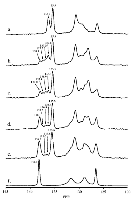
Figure 15. Phenyl region of the ^{13}\text{C} CP/MAS NMR spectra of: (a) neatame anhydrate generated by placing the original monohydrate under vacuum ( \sim 1 Torr) for three days; (b) after being sealed in a jar for two days; (c) after four days; (d) after six days; (e) after eight days; and (f) after being placed in a relative humidity environment of 84% for 12 days.
